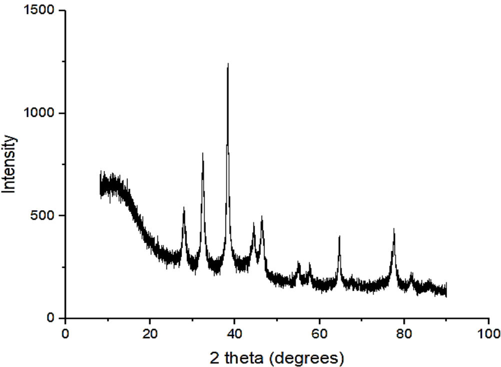
Figure 3. XRD pattern of biosynthesized silver nanoparticles from Artemisia maritima , showing characteristic peaks at 2\theta values of 27^\circ , 32^\circ , 38^\circ , 44^\circ , 46^\circ , 54^\circ , 57^\circ , 64^\circ , 67^\circ , 77^\circ , and 81^\circ , confirming their crystalline nature.
