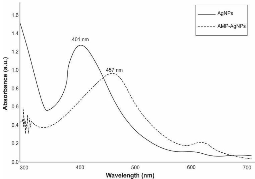
Figure 1. UV–Vis absorption spectra of biosynthesized AgNPs and ampicillin-functionalized silver nanoparticles (AMP–AgNPs). The peak at 401 nm confirms AgNP formation, while the redshift to 457 nm indicates successful ampicillin functionalization.
