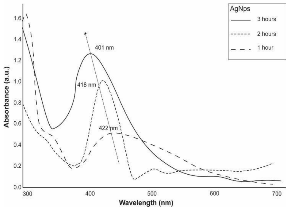
Figure 5. UV–Vis absorption spectra of AgNPs synthesized over different reaction times (1, 2, and 3 hours). The surface plasmon resonance peak shifts from 422 nm to 401 nm with longer reaction times, indicating enhanced reduction and nanoparticle formation.
