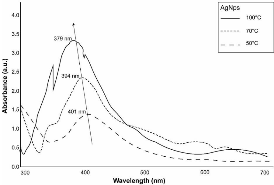
Figure 4. UV–Vis absorption spectra of AgNPs synthesized at different temperatures (50 °C, 70 °C, and 100 °C), showing a blue shift in surface plasmon resonance peaks from 401 nm to 379 nm with increasing temperature, indicating reduced particle size.
