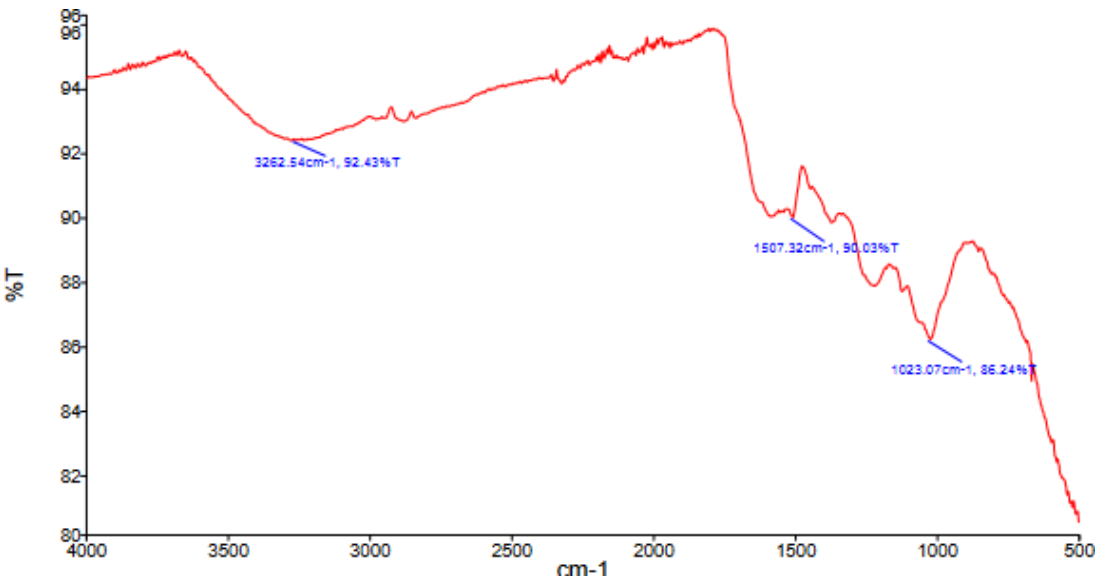
Figure 2. FTIR spectrum of Artemisia maritima -synthesized silver nanoparticles showing key absorption peaks at 3262.54 cm -1 (–OH stretch), 1507.32 cm -1 (aromatic C=C), and 1023.07 cm -1 (C–N stretch of amines), confirming the involvement of phytochemicals in nanoparticle stabilization.
